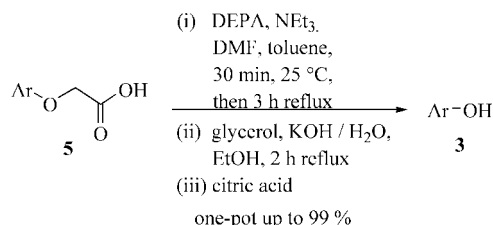
Scheme 3. Reliable deblocking sequence.
